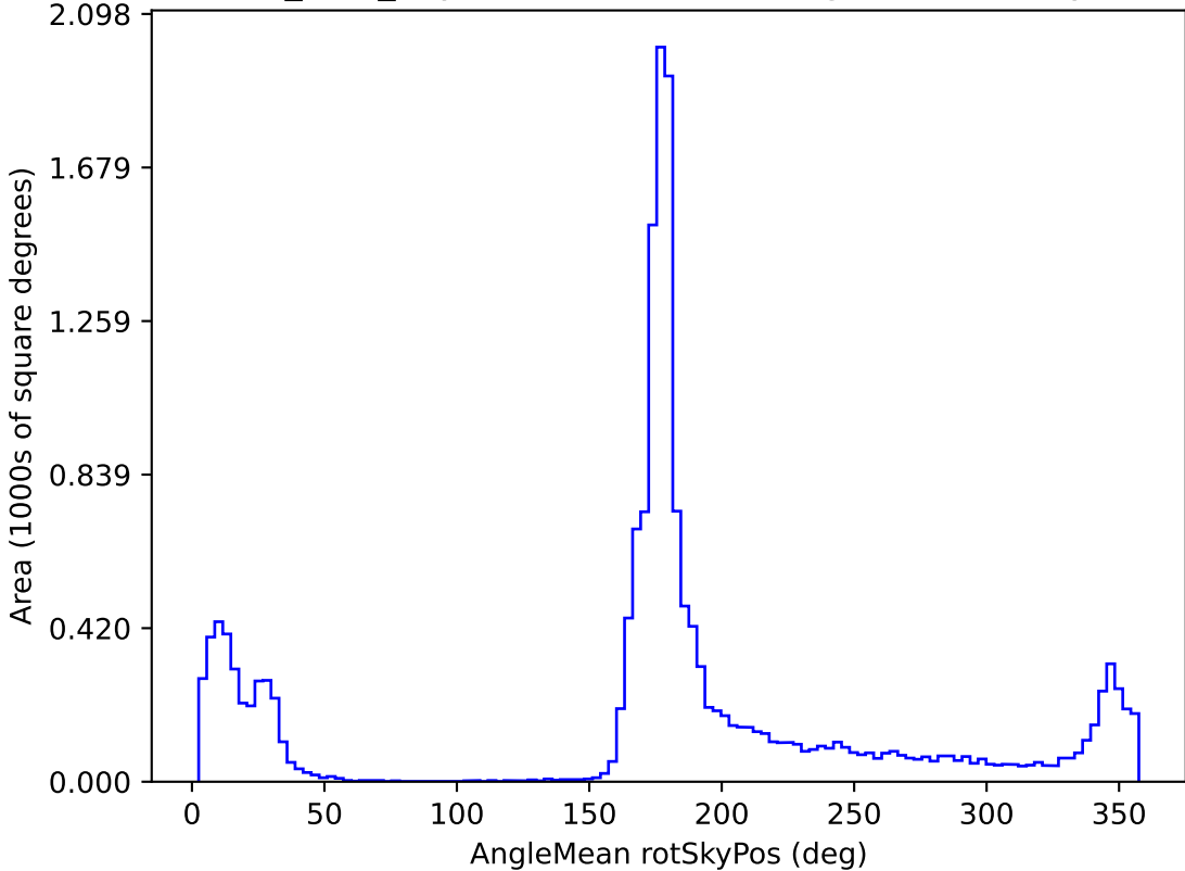
noroll_v3.4_10yrs WFD all bands: AngleMean rotSkyPos
