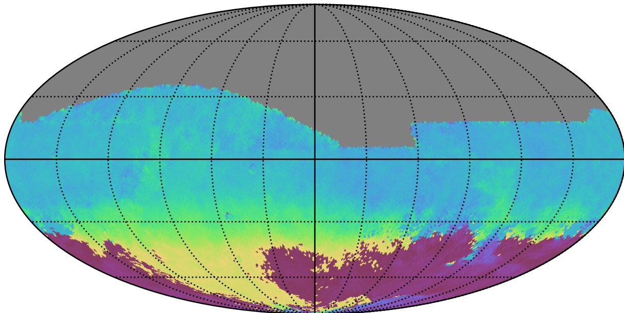
noroll_v3.4_10yrs All sky z band: AngleMean rotSkyPos
