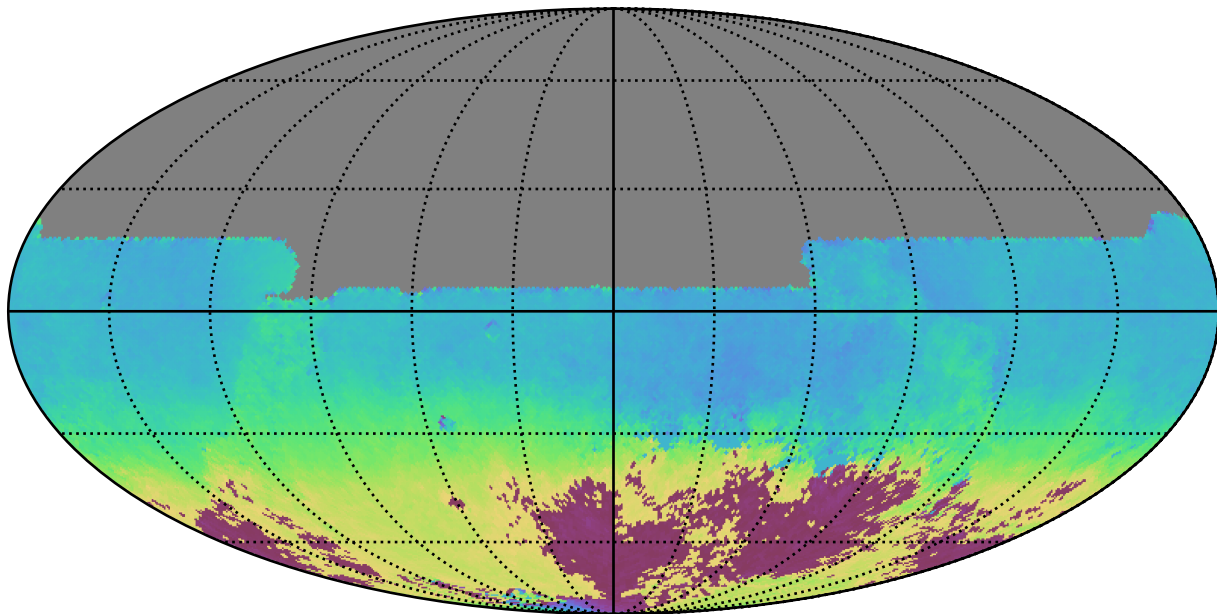
noroll_v3.4_10yrs All sky y band: AngleMean rotSkyPos
