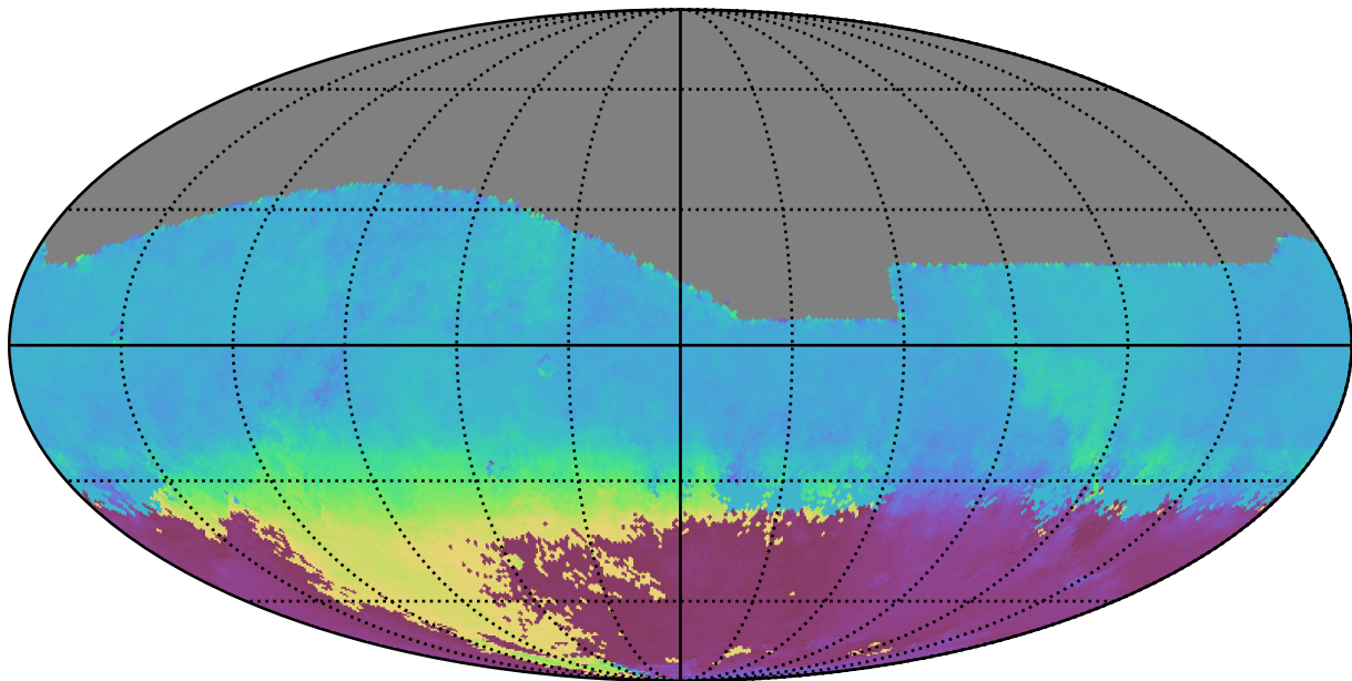
noroll_v3.4_10yrs All sky r band: AngleMean rotSkyPos
