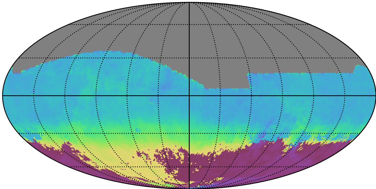
noroll_v3.4_10yrs All sky i band: AngleMean rotSkyPos
