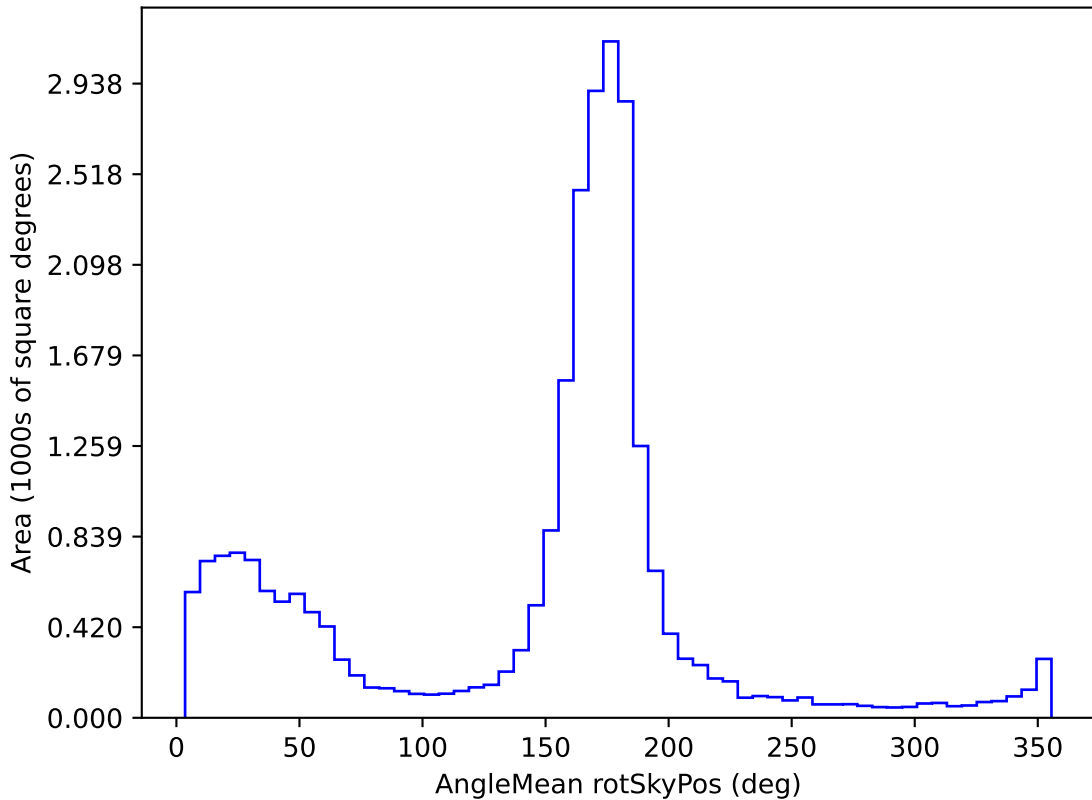
noroll_v3.4_10yrs All sky g band: AngleMean rotSkyPos
