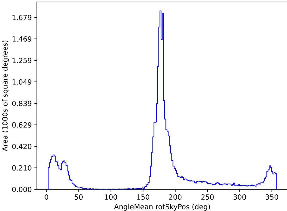
noroll_v3.4_10yrs All sky all bands: AngleMean rotSkyPos
