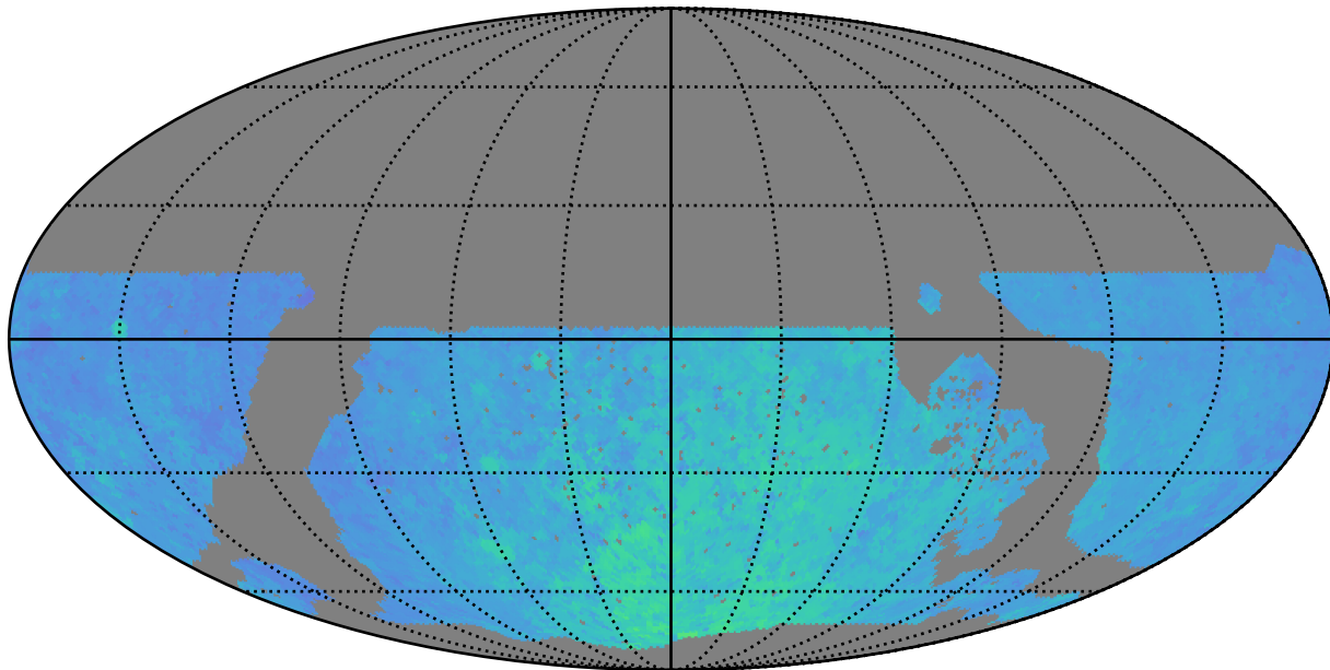
noroll_v3.4_10yrs WFD z band: 80thPercentile Season Length
