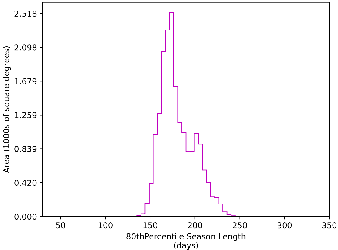
noroll_v3.4_10yrs WFD z band: 80thPercentile Season Length
