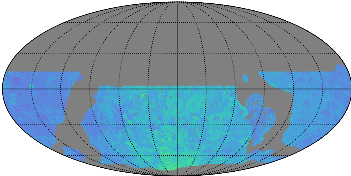
noroll_v3.4_10yrs WFD y band: 80thPercentile Season Length
