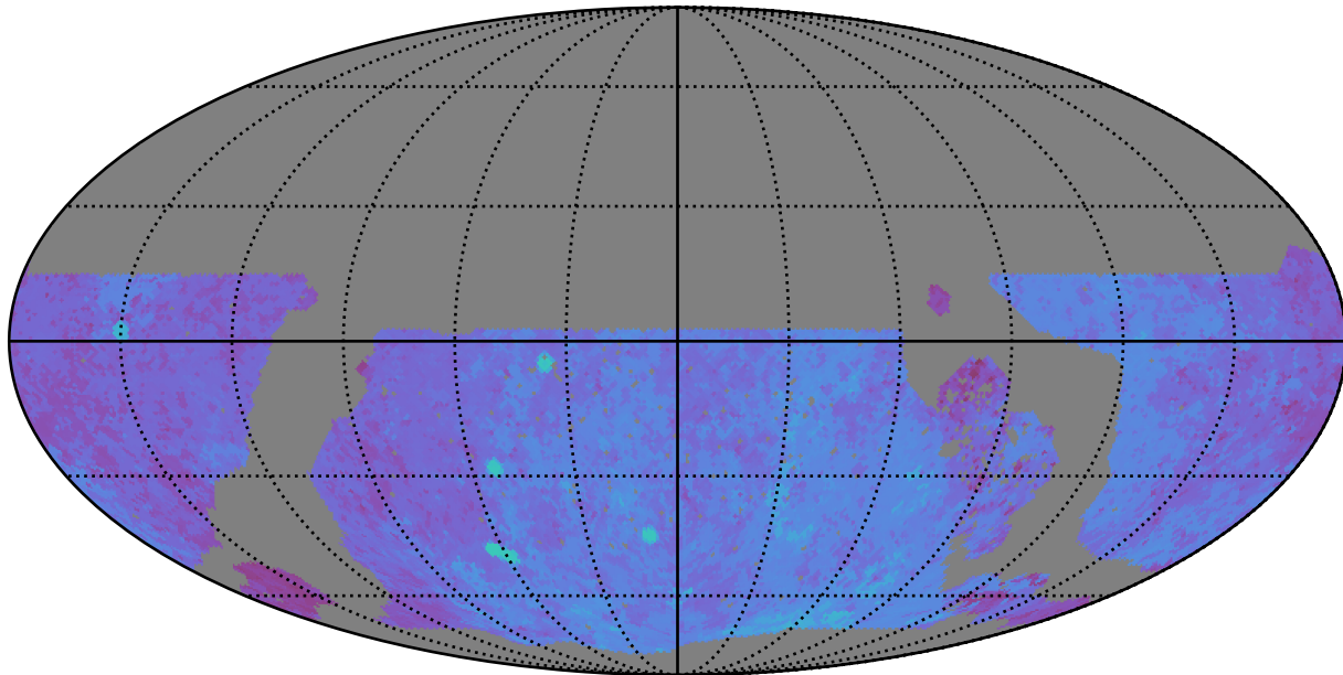
noroll_v3.4_10yrs WFD u band: 80thPercentile Season Length
