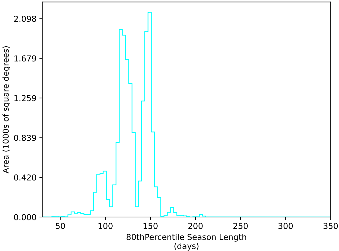
noroll_v3.4_10yrs WFD u band: 80thPercentile Season Length
