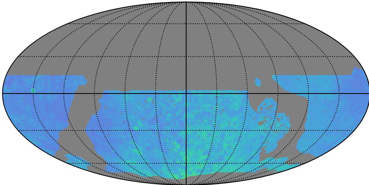
noroll_v3.4_10yrs WFD r band: 80thPercentile Season Length
