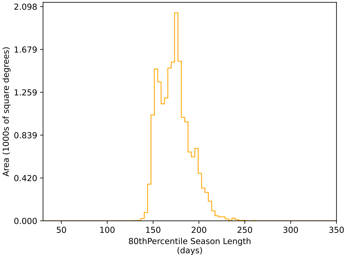
noroll_v3.4_10yrs WFD r band: 80thPercentile Season Length
