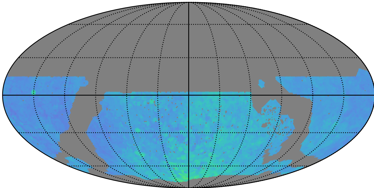
noroll_v3.4_10yrs WFD i band: 80thPercentile Season Length
