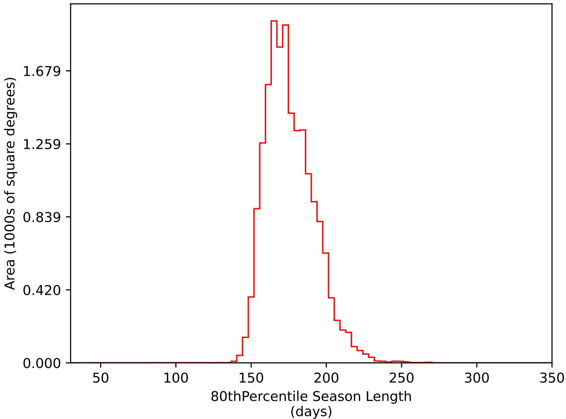
noroll_v3.4_10yrs WFD i band: 80thPercentile Season Length
