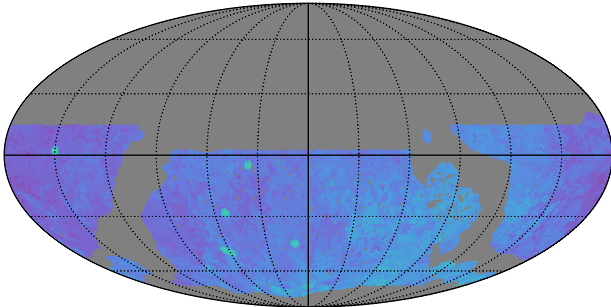
noroll_v3.4_10yrs WFD g band: 80thPercentile Season Length
