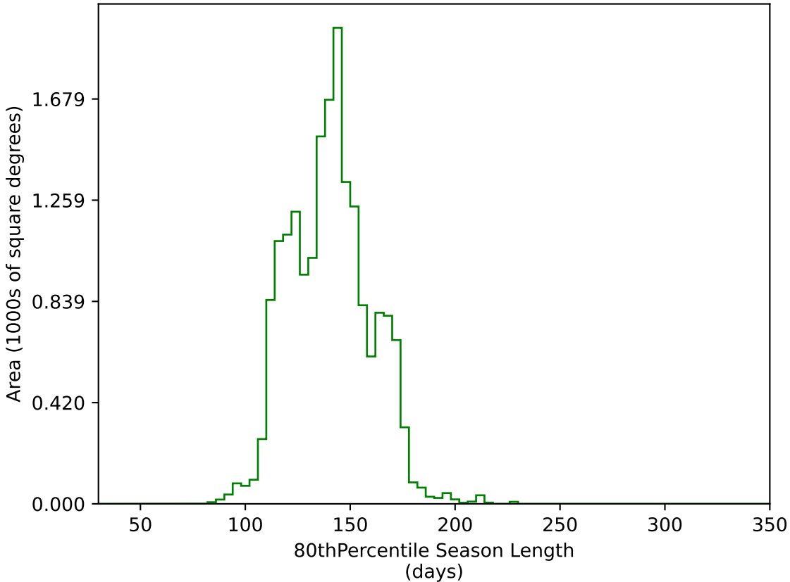
noroll_v3.4_10yrs WFD g band: 80thPercentile Season Length
