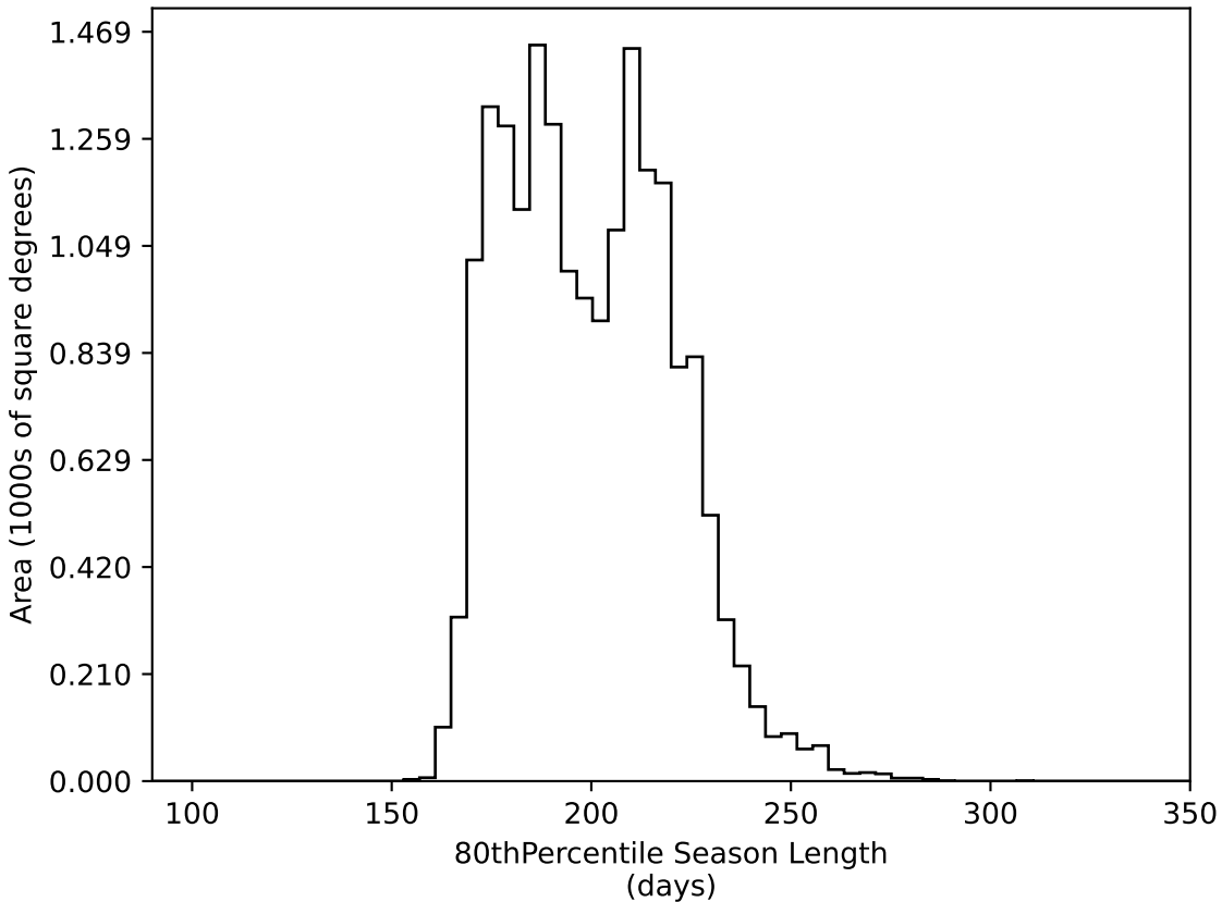
noroll_v3.4_10yrs WFD all bands: 80thPercentile Season Length
