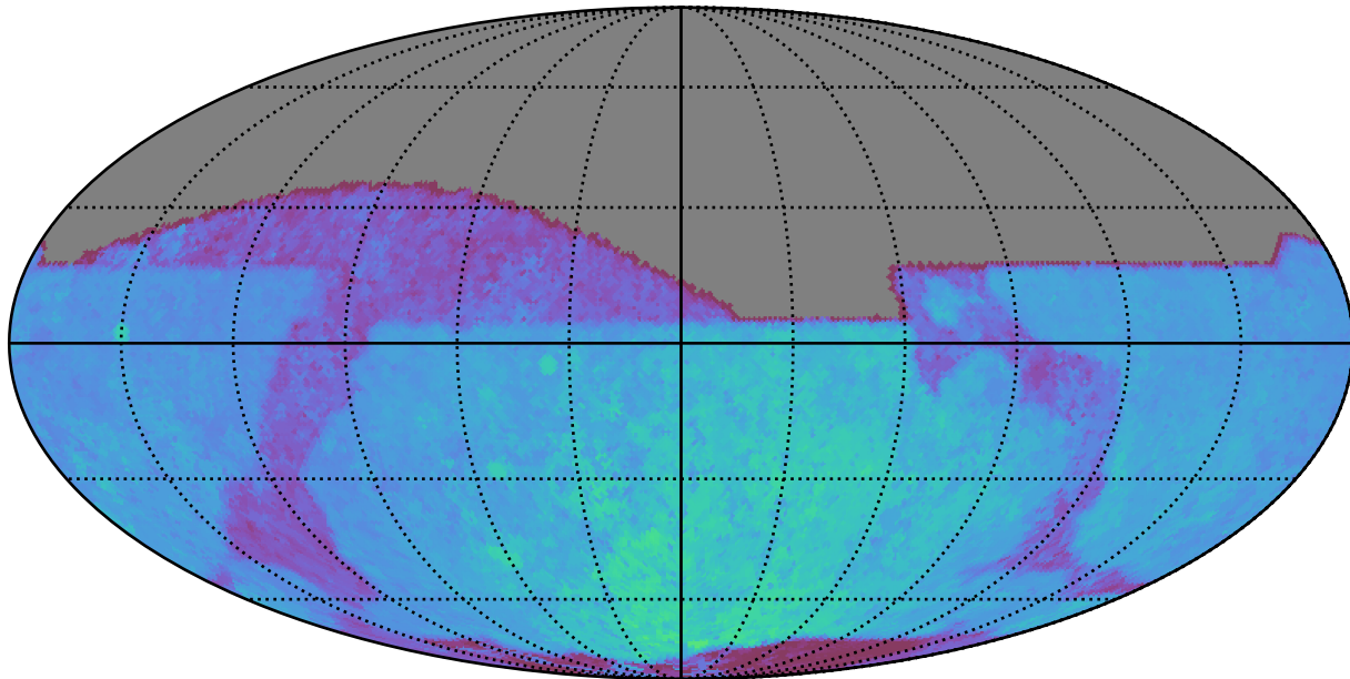
noroll_v3.4_10yrs All sky z band: 80thPercentile Season Length
