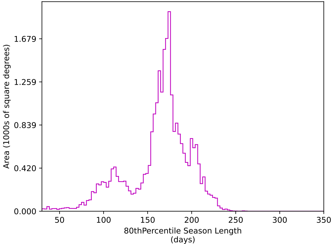
noroll_v3.4_10yrs All sky z band: 80thPercentile Season Length
