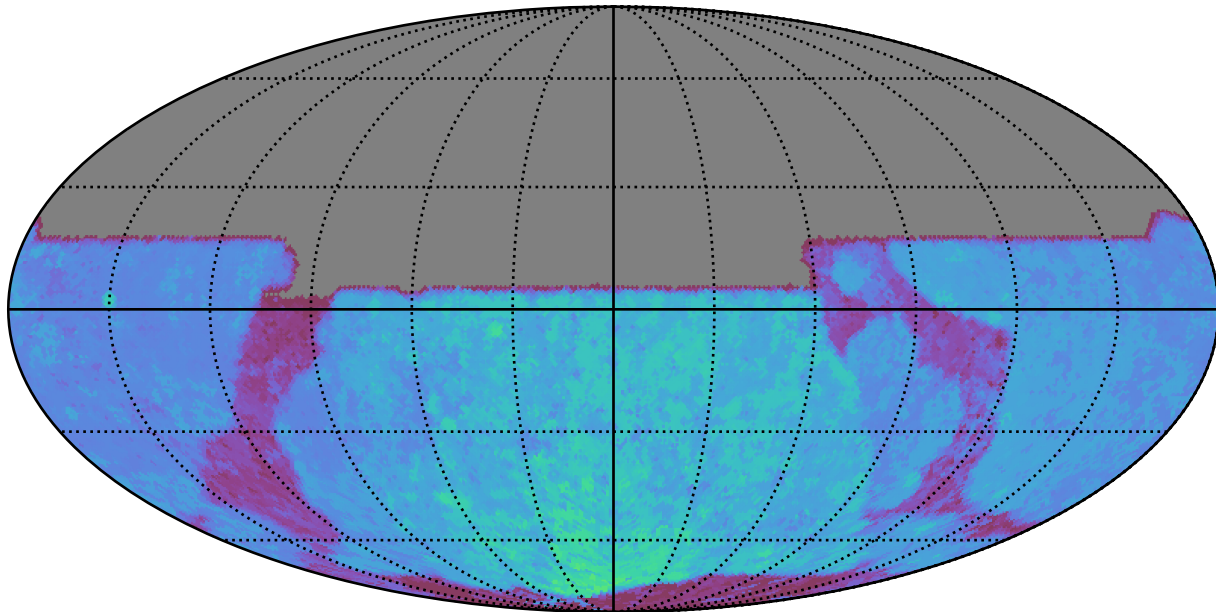
noroll_v3.4_10yrs All sky y band: 80thPercentile Season Length
