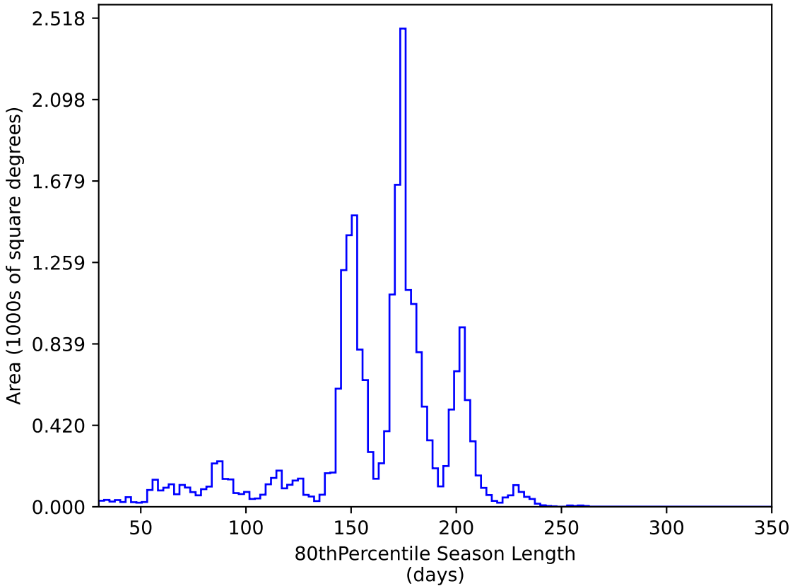
noroll_v3.4_10yrs All sky y band: 80thPercentile Season Length
