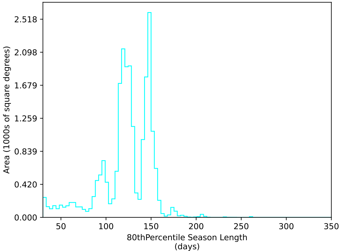
noroll_v3.4_10yrs All sky u band: 80thPercentile Season Length
