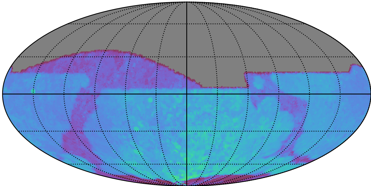
noroll_v3.4_10yrs All sky r band: 80thPercentile Season Length
