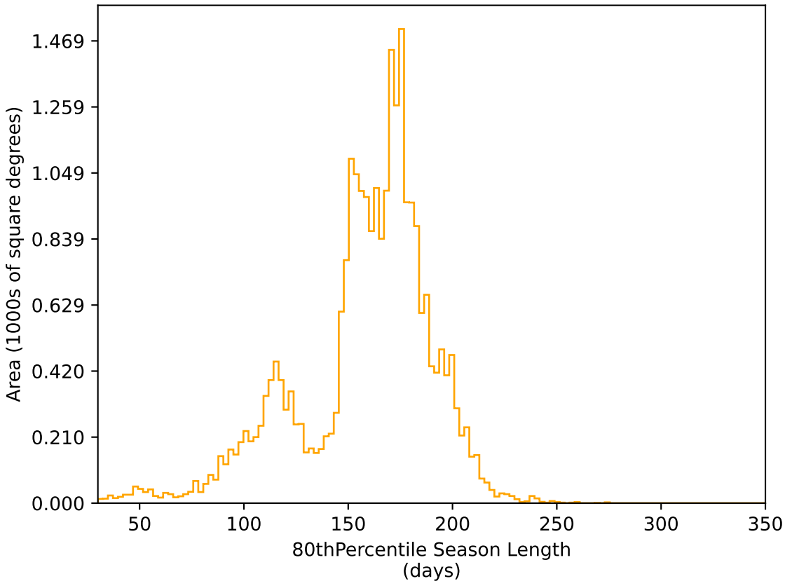
noroll_v3.4_10yrs All sky r band: 80thPercentile Season Length
