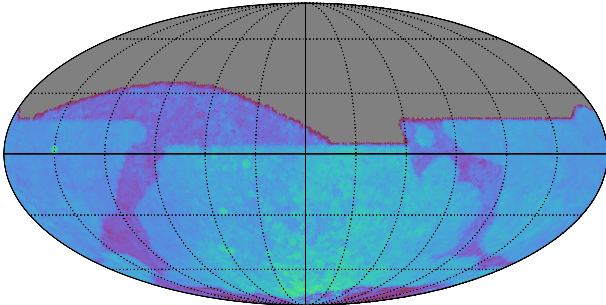
noroll_v3.4_10yrs All sky i band: 80thPercentile Season Length
