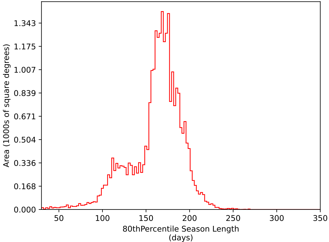
noroll_v3.4_10yrs All sky i band: 80thPercentile Season Length
