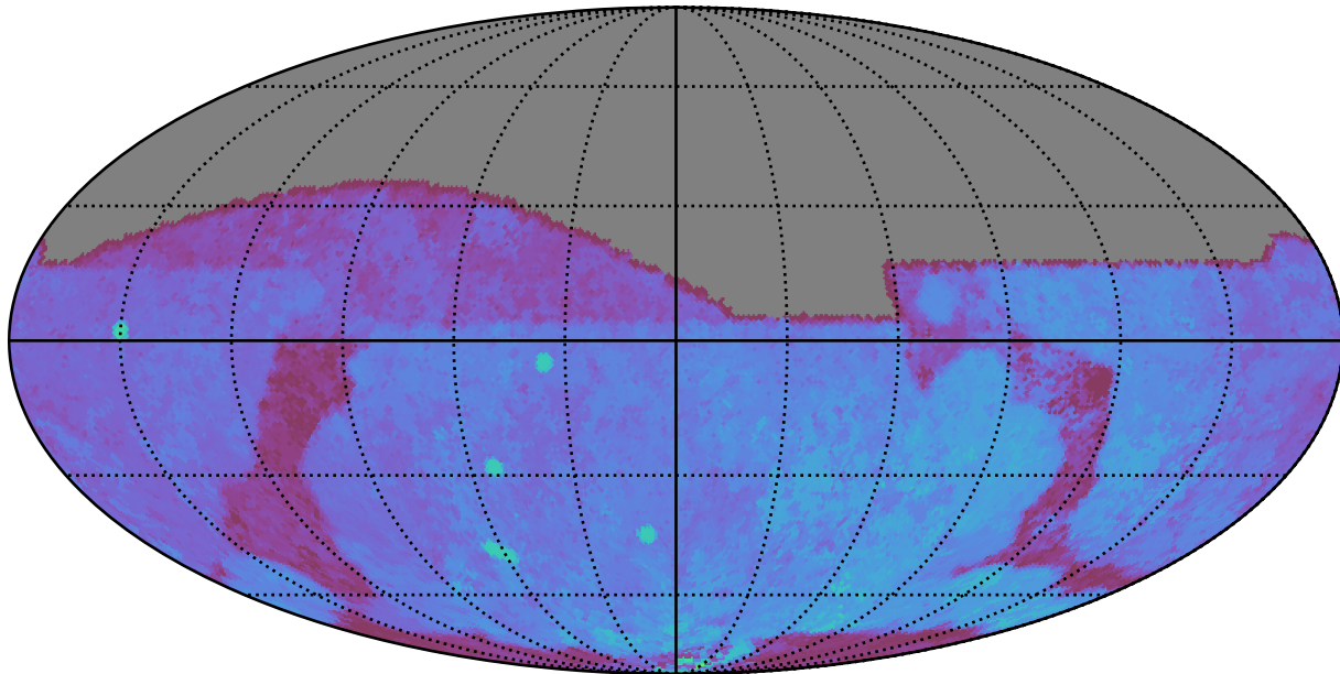
noroll_v3.4_10yrs All sky g band: 80thPercentile Season Length
