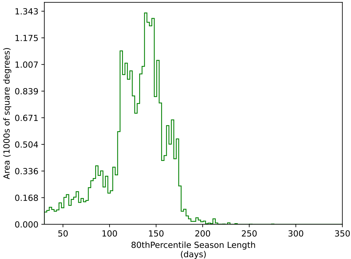
noroll_v3.4_10yrs All sky g band: 80thPercentile Season Length
