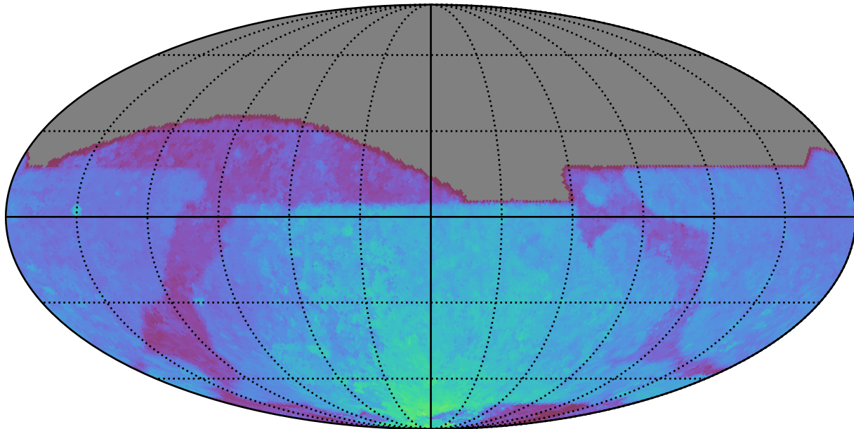
noroll_v3.4_10yrs All sky all bands: 80thPercentile Season Length
