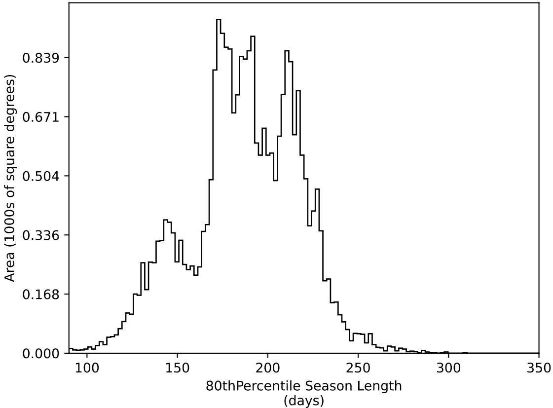
noroll_v3.4_10yrs All sky all bands: 80thPercentile Season Length
