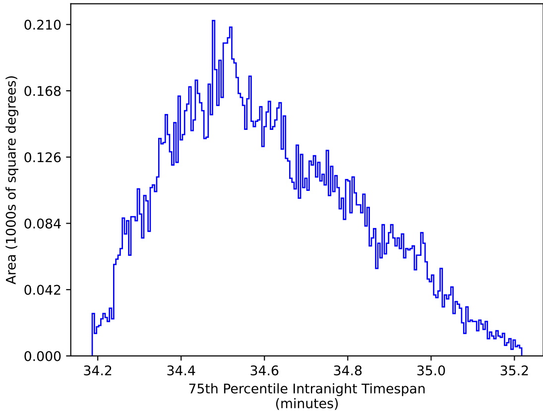
noroll_v3.4_10yrs WFD zy bands: 75th Percentile Intranight Timespan
