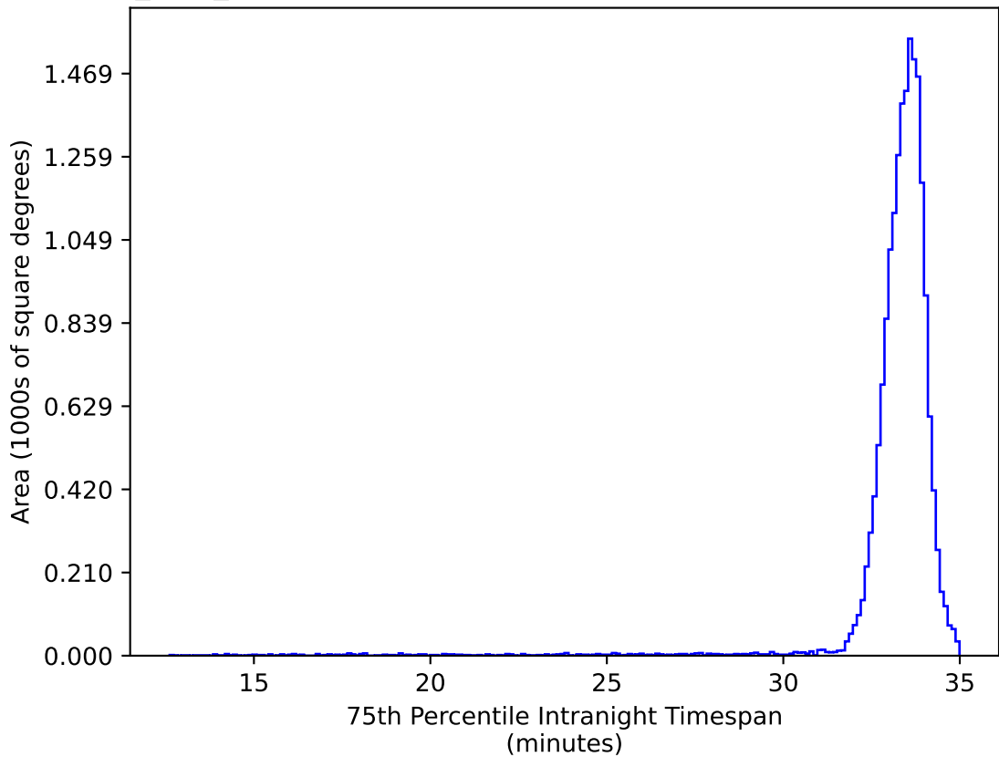
noroll_v3.4_10yrs WFD ug bands: 75th Percentile Intranight Timespan
