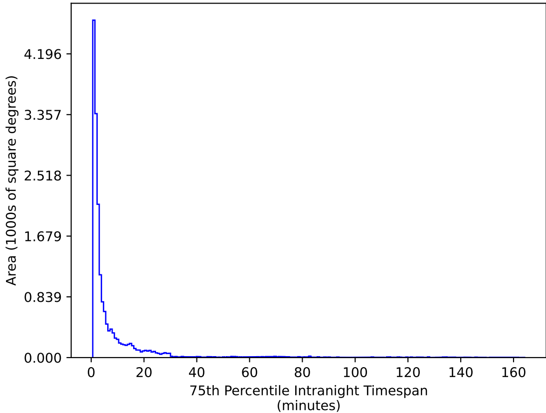
noroll_v3.4_10yrs WFD u band: 75th Percentile Intranight Timespan
