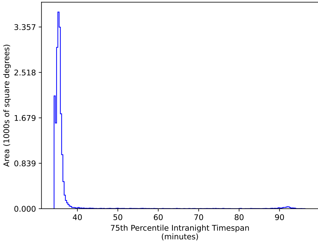
noroll_v3.4_10yrs WFD ri bands: 75th Percentile Intranight Timespan
