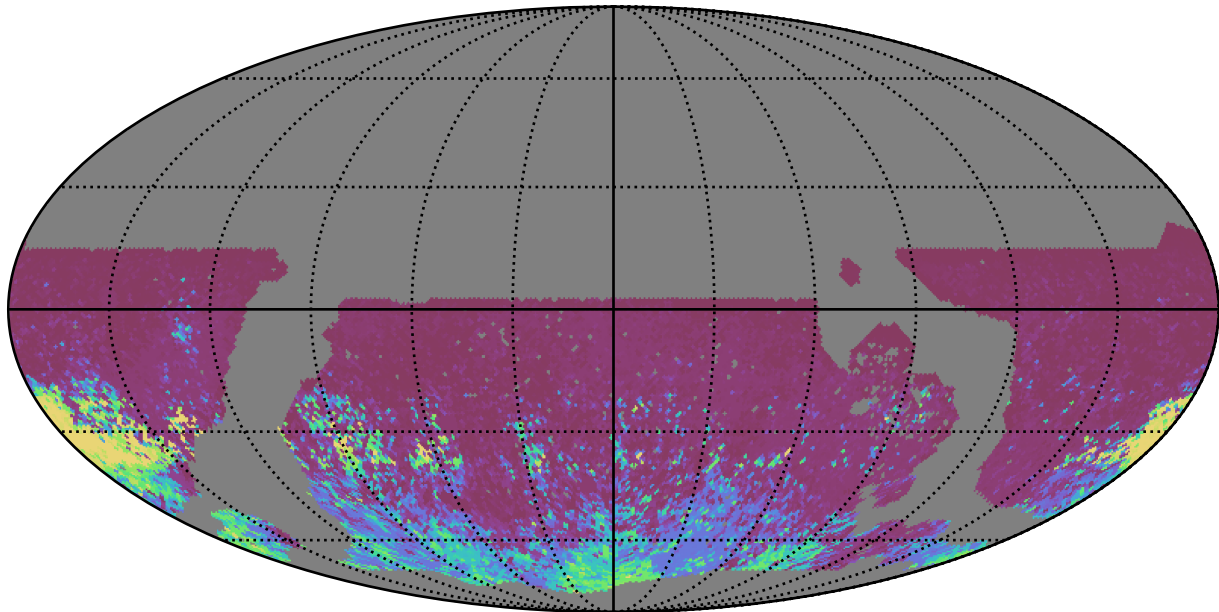
noroll_v3.4_10yrs WFD r band: 75th Percentile Intranight Timespan
