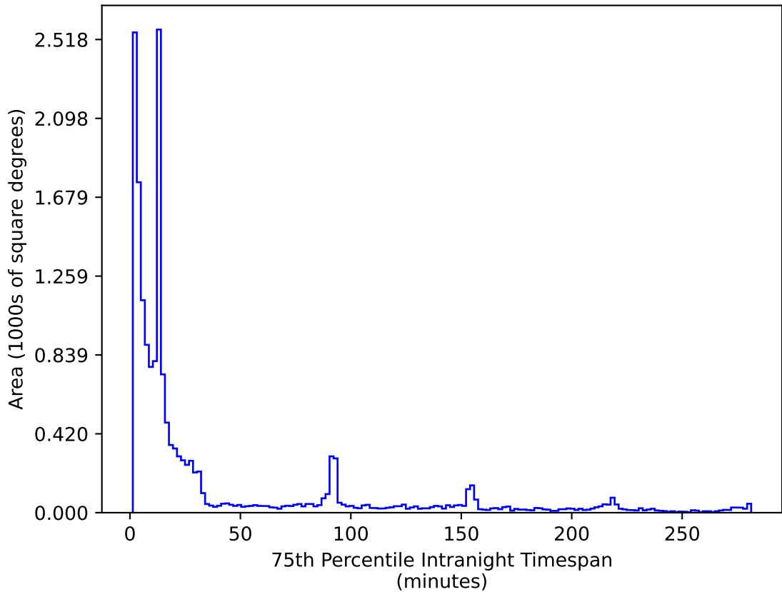
noroll_v3.4_10yrs WFD r band: 75th Percentile Intranight Timespan
