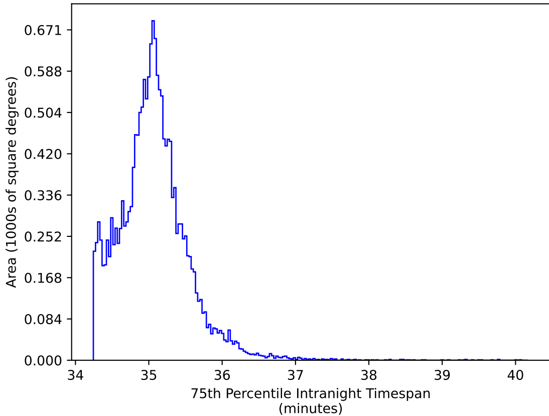
noroll_v3.4_10yrs WFD iz bands: 75th Percentile Intranight Timespan
