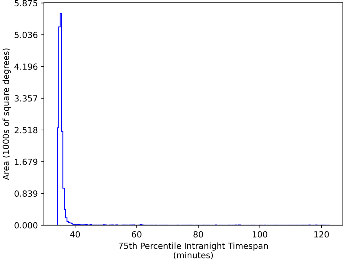
noroll_v3.4_10yrs WFD gr bands: 75th Percentile Intranight Timespan
