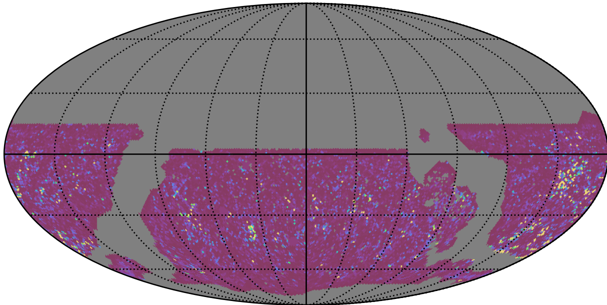
noroll_v3.4_10yrs WFD g band: 75th Percentile Intranight Timespan
