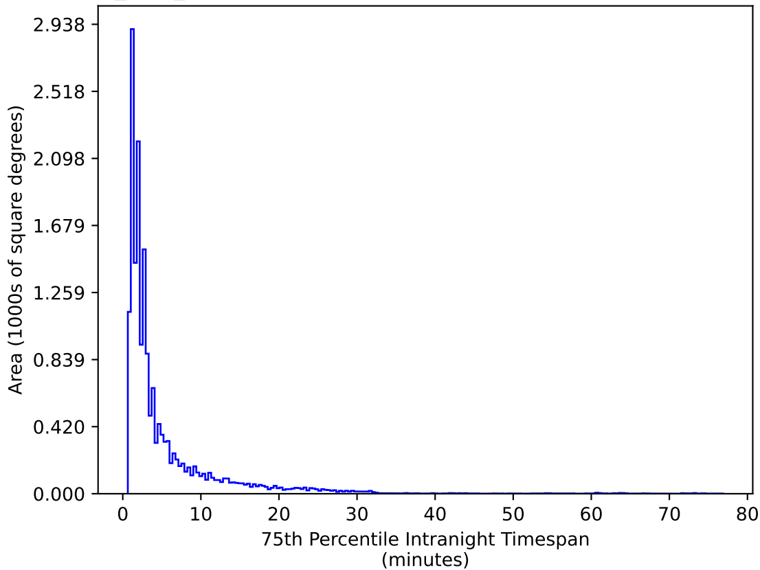
noroll_v3.4_10yrs WFD g band: 75th Percentile Intranight Timespan
