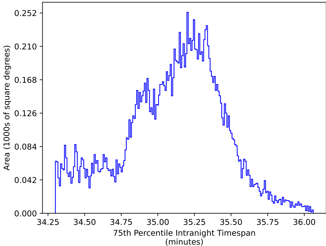
noroll_v3.4_10yrs WFD all bands: 75th Percentile Intranight Timespan
