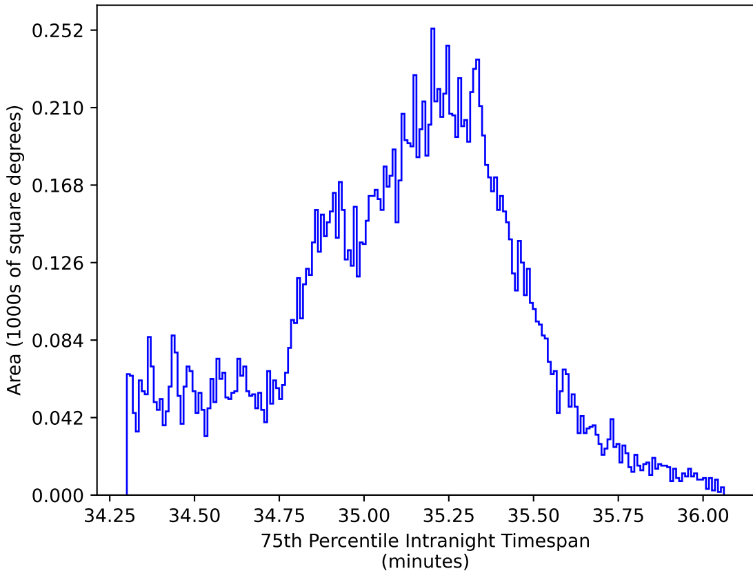
noroll_v3.4_10yrs WFD: 75th Percentile Intranight Timespan
