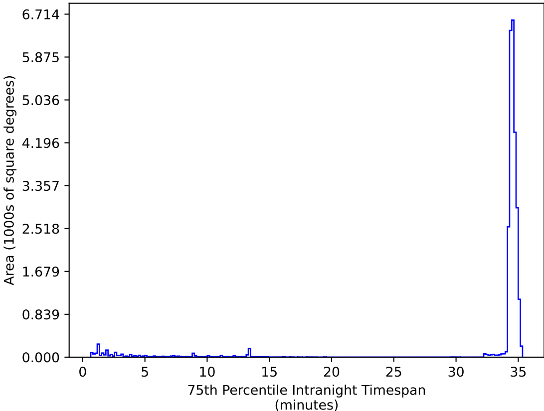
noroll_v3.4_10yrs All sky zy bands: 75th Percentile Intranight Timespan
