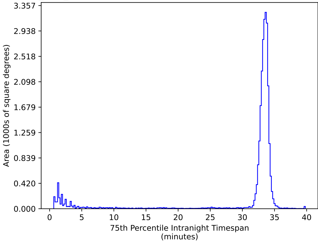
noroll_v3.4_10yrs All sky ug bands: 75th Percentile Intranight Timespan
