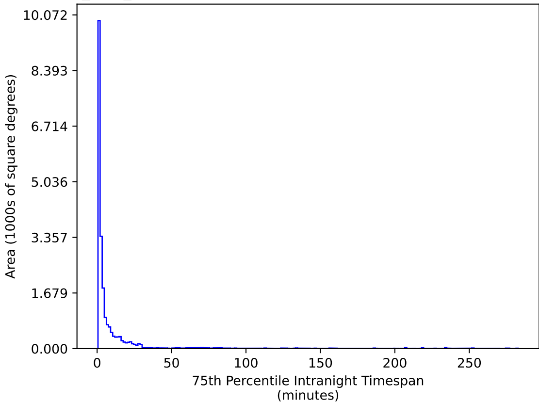
noroll_v3.4_10yrs All sky u band: 75th Percentile Intranight Timespan
