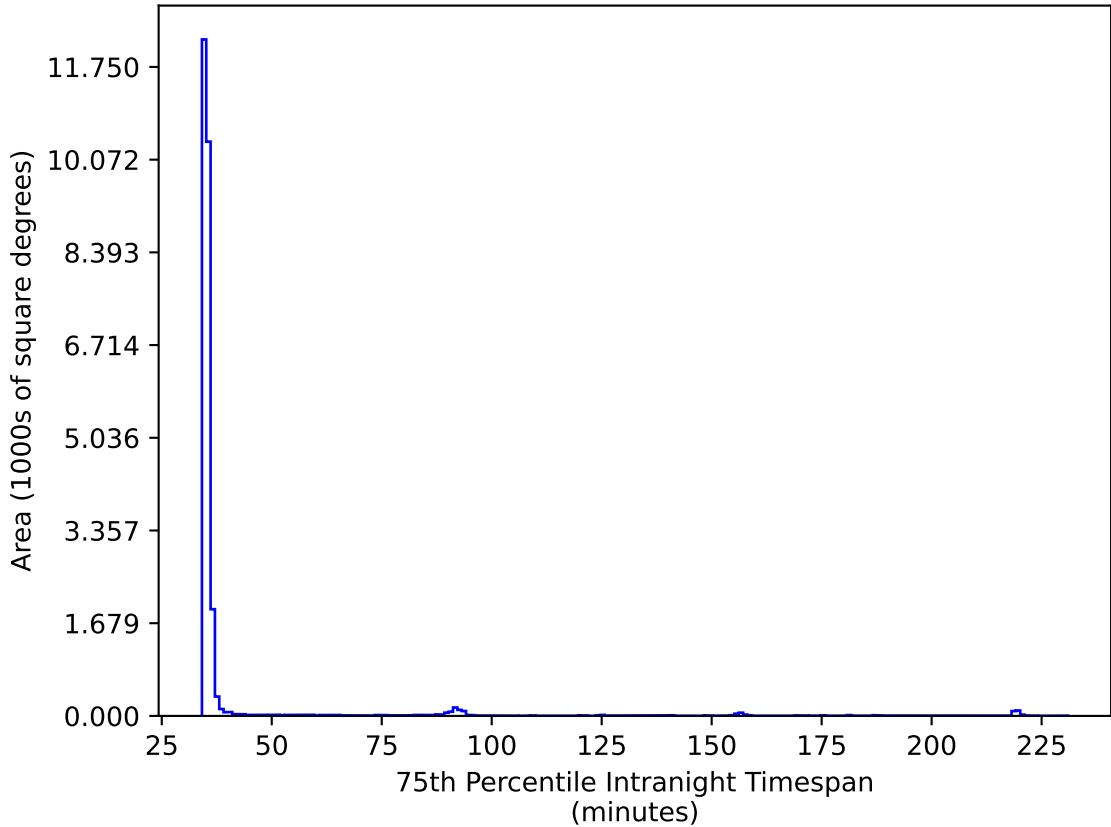
noroll_v3.4_10yrs All sky ri bands: 75th Percentile Intranight Timespan
