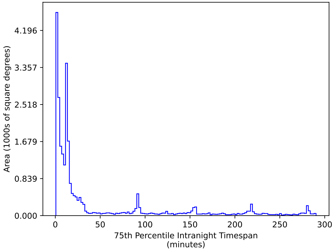
noroll_v3.4_10yrs All sky r band: 75th Percentile Intranight Timespan
