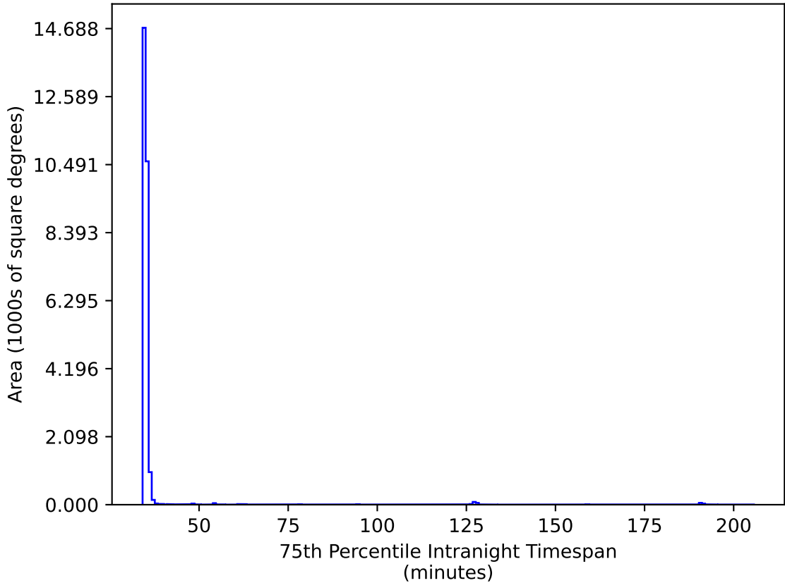
noroll_v3.4_10yrs All sky iz bands: 75th Percentile Intranight Timespan
